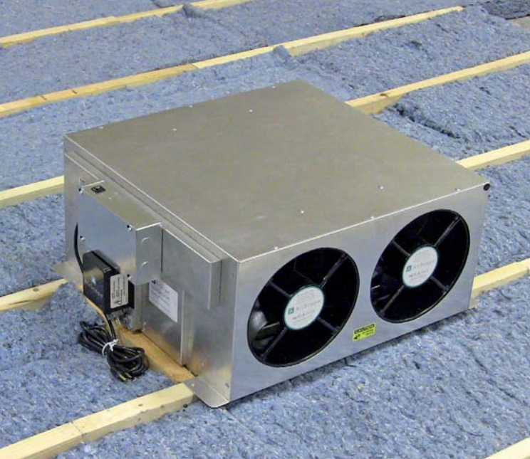
An attic-mounted whole-house fan pulls hot air into the attic space (where it exits through vents) while drawing cooler nighttime air into the living-space through open windows.
